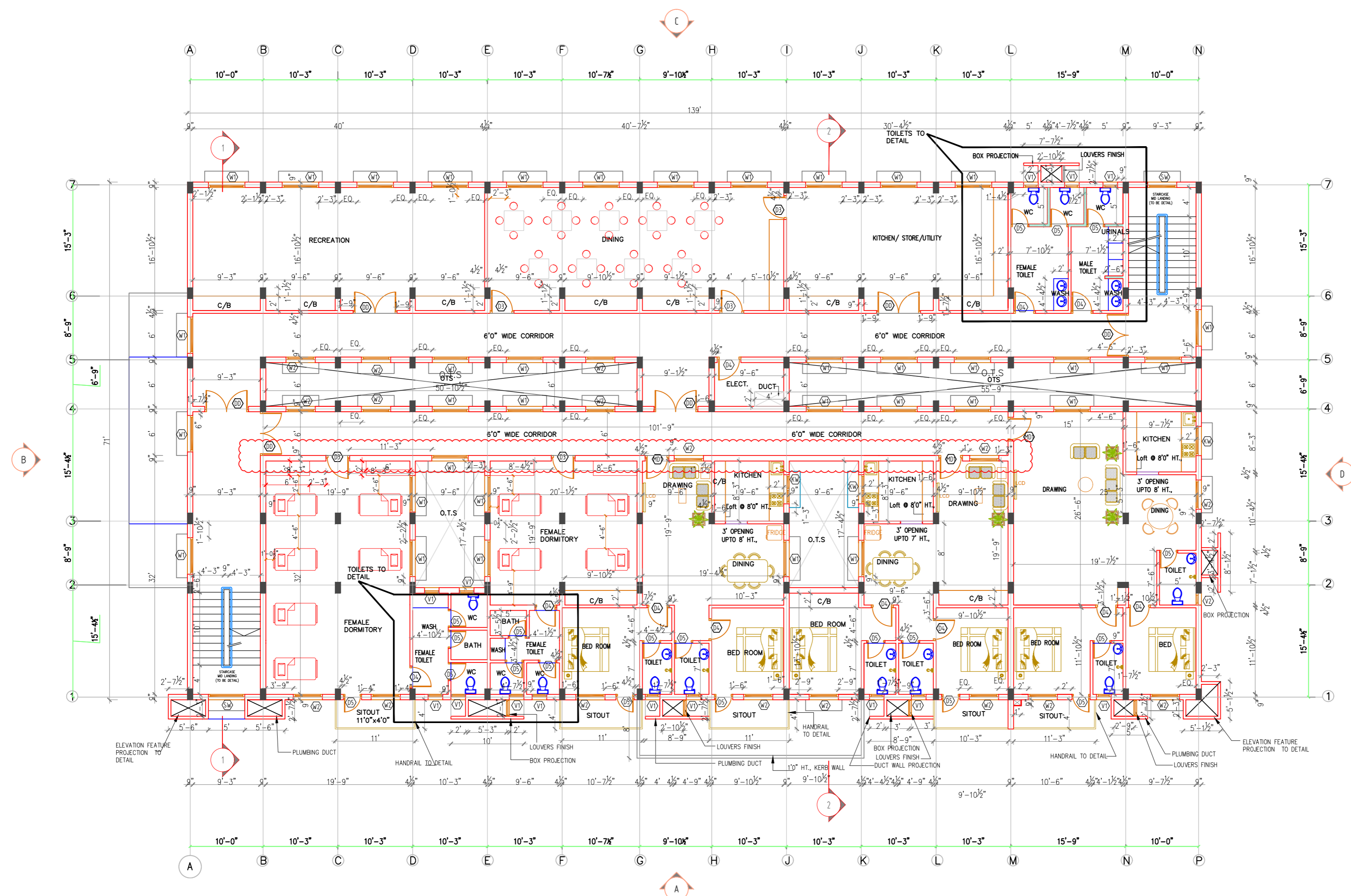
FIRST FLOOR PLAN 1 RURAL BLOCK SCALE: 1:100
